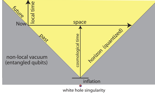
FIG. 1. Schematic of the Horizon Model. The non-local region inside the vacuum had instantaneously inflated to a size (dia) of \sim 10^{-26}m before spacetime began .
