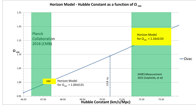
FIG. 2. Horizon Model (HM) values of the Hubble constant as a function of \Omega_{vac} . ( P=\Omega_{vac} when \rho_{local} = \rho_{crit} ) With \Omega_{vac} = \Omega = 1.00 \pm 0.01 , the HM value for H ( 67.87 \pm 0.38 ) agrees very well with the Planck collaboration measurement. The HM values for H are in agreement with the SH0ES team measurement if \Omega_{vac} = 1.16 \pm 0.03 . For a Hubble time of 13.8 Gyr, \Omega_{vac} = 1.094 .
